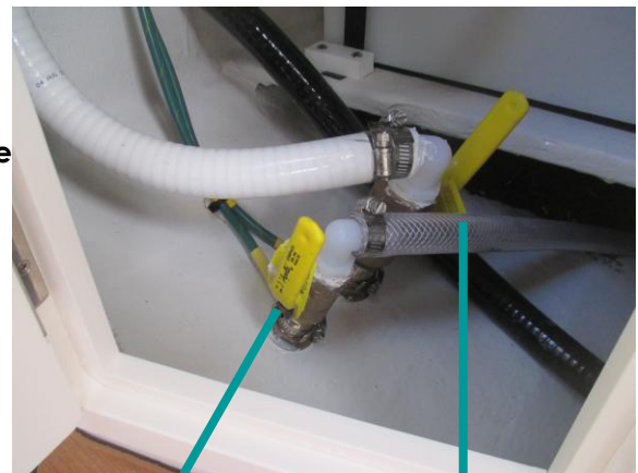
Intake Valve (open)
