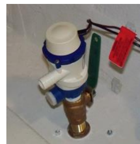
Livewell Pump Assembly in the "OPEN" Position
